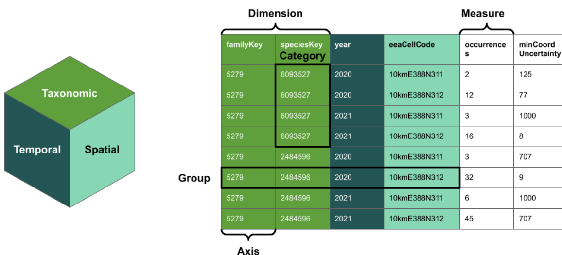
Figure 1: Schematic representation of a cube.
