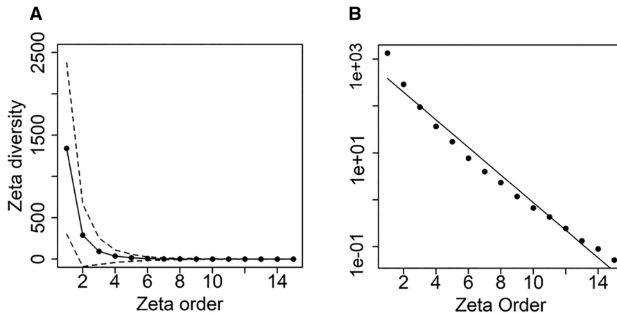
Figure 3. Zeta diversity decline of African vascular plants fitted using 23,189 species with 10,000 random site combinations for orders 1–15. A, the solid line reflects the quantified relationship between the zeta diversity and the different orders of zeta, bounded by the zeta values of the standard deviation. B, the form of the decline, corresponding to the exponential fit.
